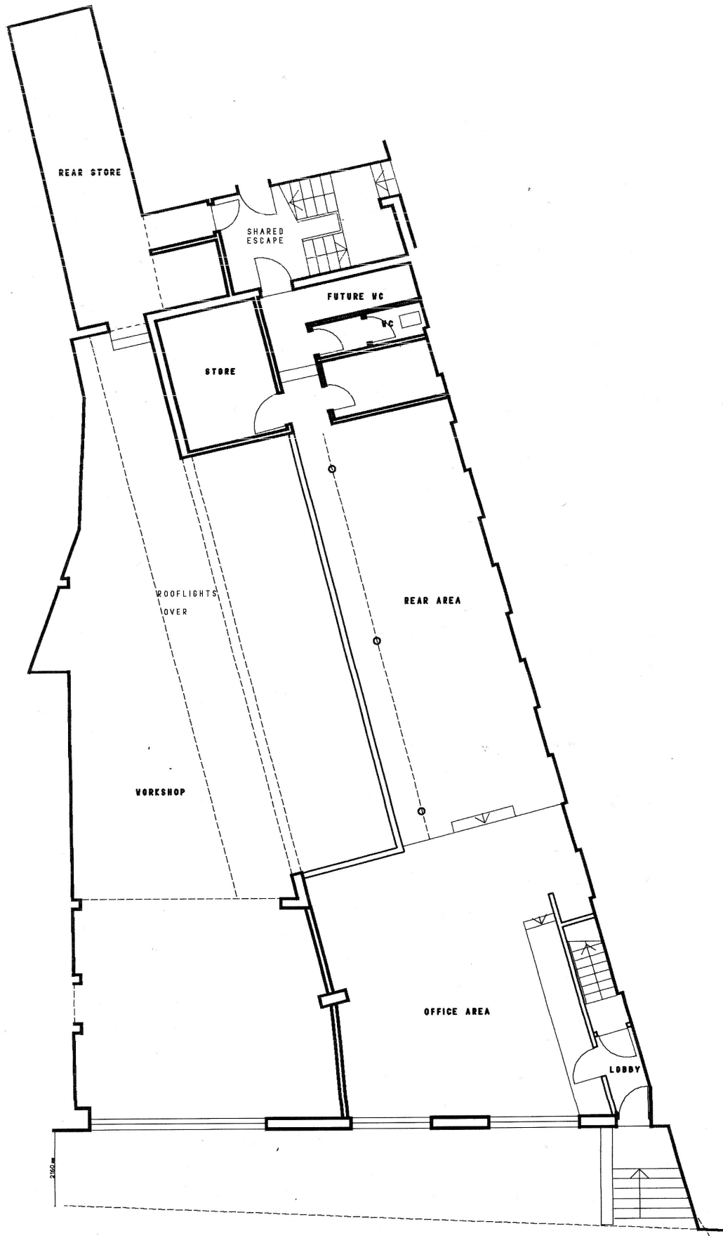
1A EMBANKMENT PUTNEY EXISTING GROUND FLOOR PLAN
